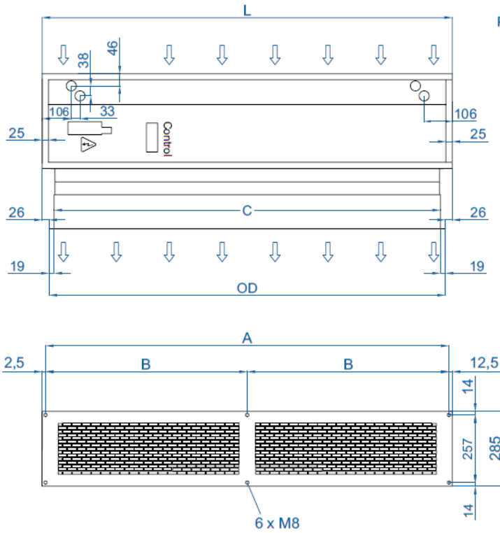
Installation horizontale
