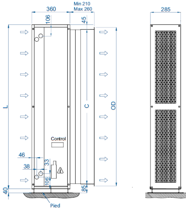
Installation verticale
